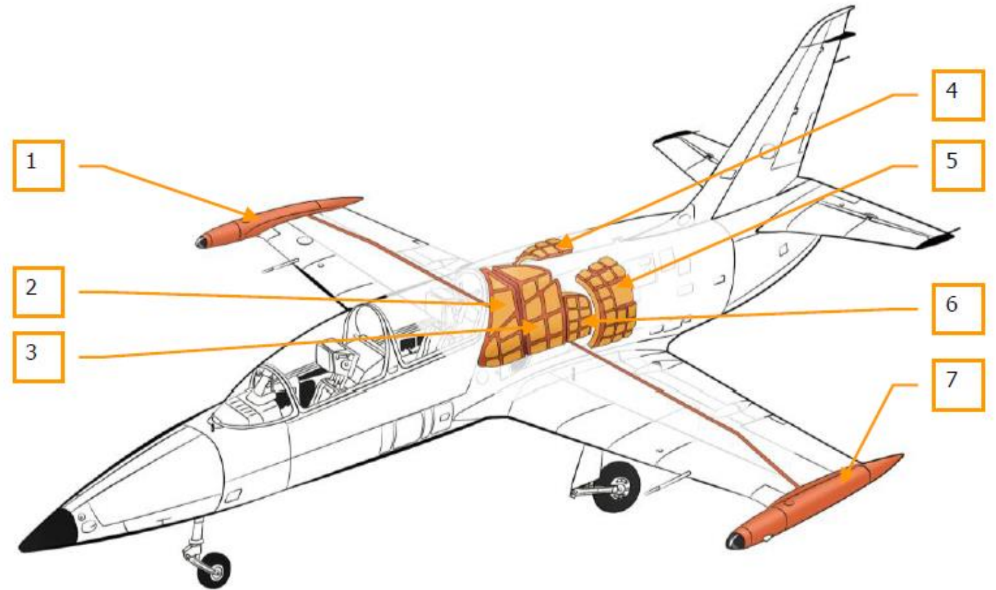
Figure 63: Fuel tanks
